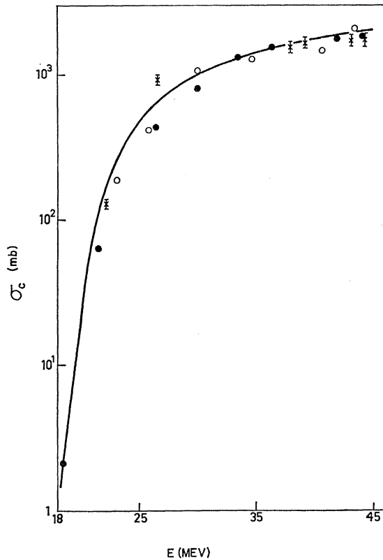
FIG. 62. Comparison of \text{U} excitation function data with the computed curve for \sigma_e from Fig. 59, providing an example of a typical fit for a heavy element, using a potential derived from analysis of elastic scattering data. \circ , \text{U}^{233} ; \bullet , \text{U}^{235} ; \times , \text{U}^{238} .
