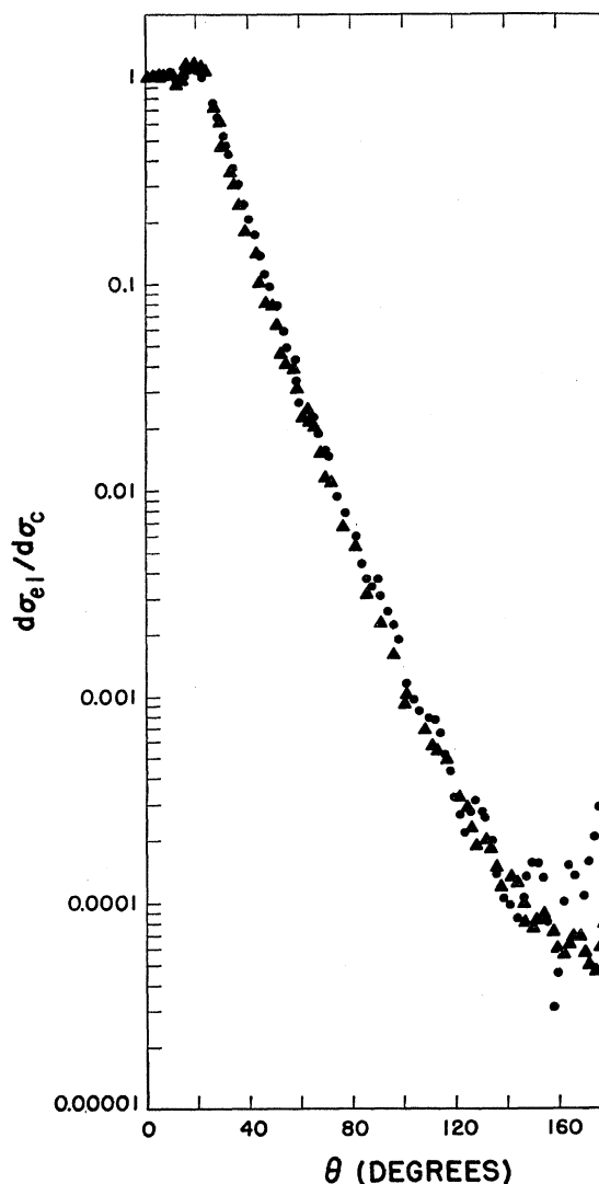
FIG. 71. Plots analogous to those in Fig. 79 for a "realistic" surface ( d = 0.5 \times 10^{-13} cm). V = 60 Mev; W = 15 Mev; d = 0.5 \times 10^{-13} cm; \Delta , exact; \bullet , \text{Re } \delta = 0 .
