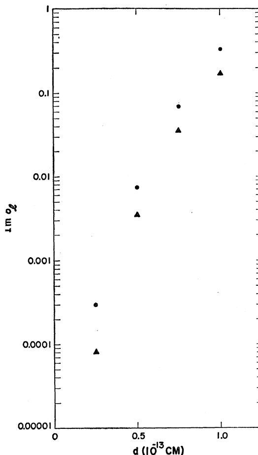
FIG. 76. Plot analogous to Fig. 75 for two large angular momenta. V=60 Mev; W=15 Mev; \bullet , l=28 ; \Delta , l=29 .
