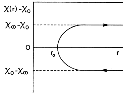
FIG. 28. Coordinate angle \chi(r) - \chi_0 as a function of radial position r along the orbit as indicated in Fig. 24.
