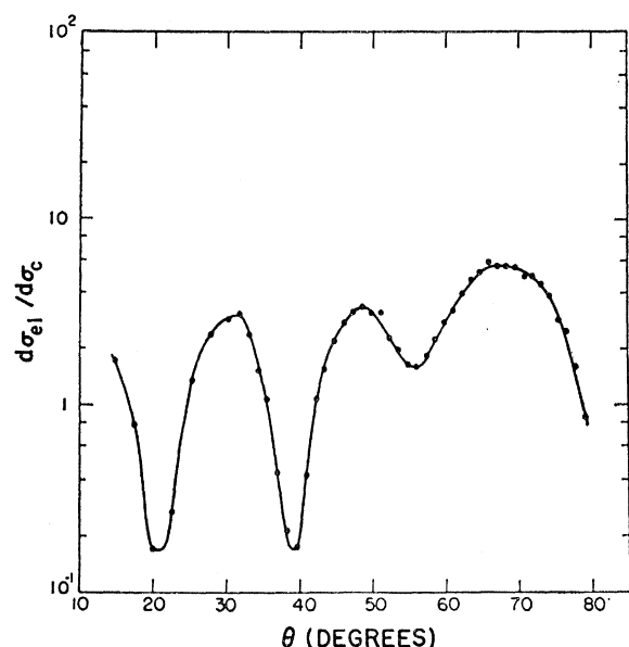
FIG. 41. Ratio of the differential scattering cross section to the Coulomb cross section for 40-Mev alpha particles incident on C. C(\alpha, \alpha)C .
