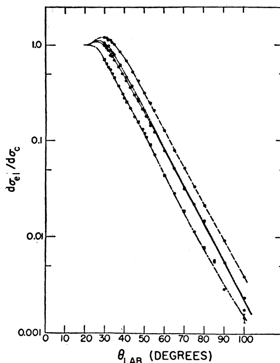
FIG. 20. Ratios of the experimental differential cross sections to the Coulomb cross section as a function of scattering angle for 40-Mev alpha particles on Ta, ---; Au, —; Pb, .....; and Th, — · —.
