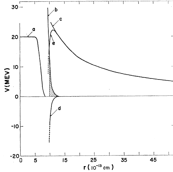
FIG. 63. Nuclear charge density (curves a and b—the latter expanded) of \text{U} obtained in electron scattering experiments along with the Coulomb potential curve (curve c) and the nuclear potential tail (curve d) as well as the nuclear plus Coulomb potential (curve e) in the tail region.
