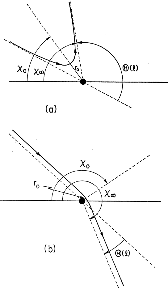
FIG. 24. Scattering geometry for (a) an attractive and (b) a repulsive potential. The classical turning point radius r_0 and angle \chi_0 are shown along with the final asymptote angle \chi_\infty and the deflection angle \Theta(l) .
