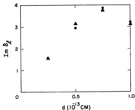
FIG. 75. Imaginary part \text{Im } \delta_l of the nuclear phase shift as a function of surface diffuseness distance d for two small angular momenta. V=60 Mev; W=15 Mev; \Delta , l=0 ; \bullet , l=1 .
