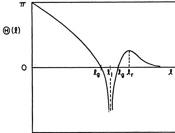
FIG. 31. Classical deflection function \Theta(l) as a function of angular momentum l for a repulsive potential. The rainbow angular momentum l_r , the orbiting angular momentum l_1 , and the glory angular momentum l_g are indicated.
