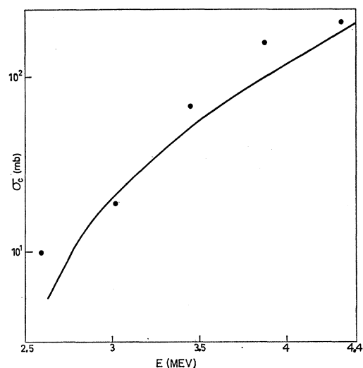
FIG. 61. Comparison of the (\alpha, n) reaction cross section of Mg with the appropriate computed curve for \sigma_c from Fig. 59. Igo argues that the (\alpha, n) reaction makes up most of \sigma_c in this energy range. The potential resulting from fitting the elastic scattering data leads also to good agreement for the reaction data.
