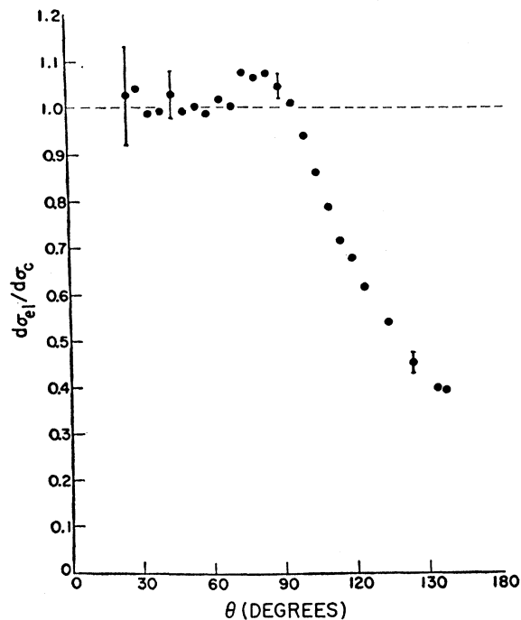
FIG. 9. Ratio to the Coulomb cross section of the differential cross section for the elastic scattering of 22-Mev alpha particles by Pb as a function of the scattering angle.
