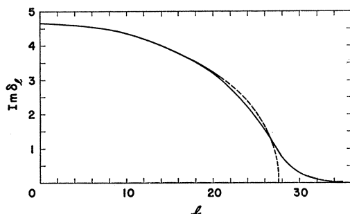
FIG. 77. \text{Im } \delta_l calculated classically for a straight line orbit intersecting a Saxon density form, as a function of angular momentum. l_0 = 1 \times 10^{-13} cm; — — —, d=0 ; —, d=0.5 \times 10^{-13} cm.
