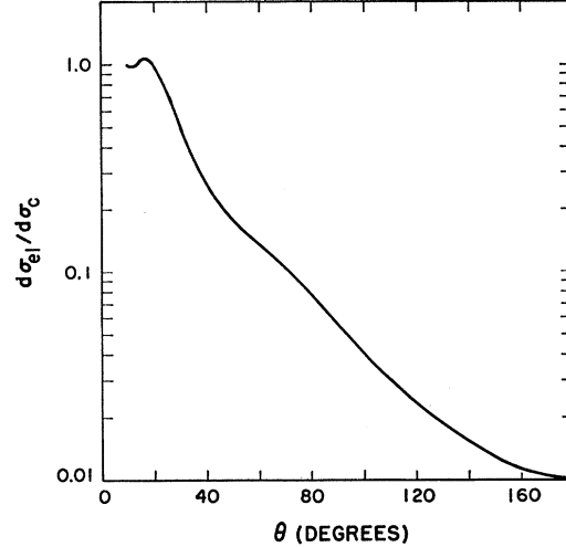
FIG. 67. A typical angular distribution (ratio to Coulomb) for a potential with a large imaginary part. The back scattering drops only two orders of magnitude, indicating that the imaginary part causes considerable back reflection. V=0 ; W=200 Mev; d=0.5 \times 10^{-13} cm.
